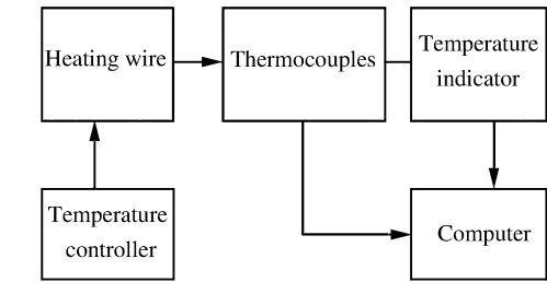
图 2 慢烤实验系统示意图 Fig. 2 System sketch of slow cook-off experiment
