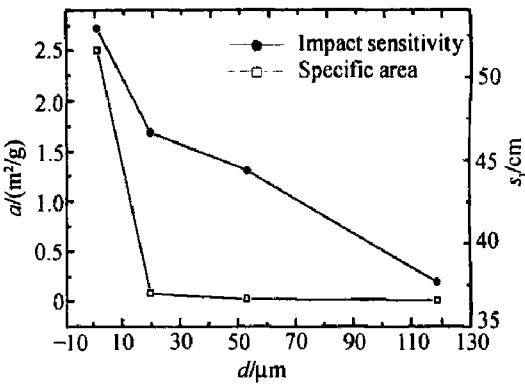
图 4 RDX 粒度、比表面积和撞击感度关系曲线 Fig.4 The curve of impact sensitivity particle size and specific area of RDX
