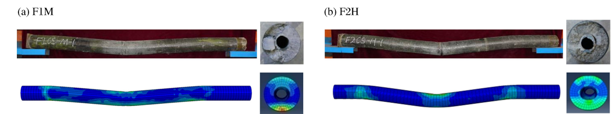
图 2 试验与模拟变形模态对比 Fig. 2 Comparison between test and simulated deformation modes
