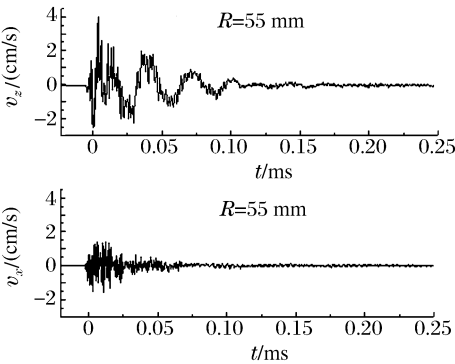
图 3 A 点无隔振沟振动波形 Fig.3 The vibration waves without trench
