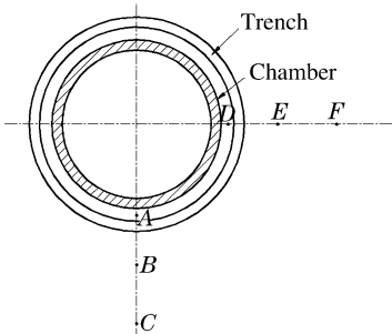
图 2 测点布局 Fig.2 Arrangement of the measuring points
