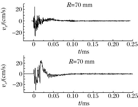
图 4 A 点有隔振沟振动波形 Fig.4 The vibration waves with trench
