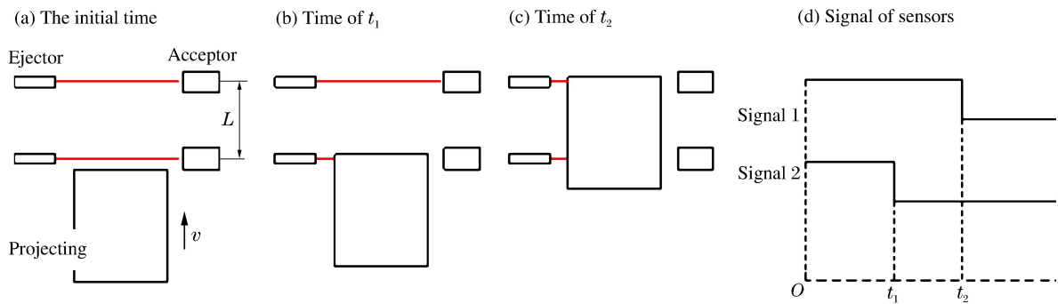
图 5 抛射筒发射速度的非接触式测量方法 Fig. 5 Uncontacted method for measuring speed of projecting cylinder
