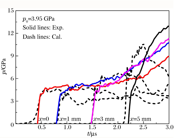
图 7 CL-20/FOX-7 混合炸药计算与实验结果对比 Fig. 7 Experimental and calculated pressure histories in shock initiation of CL-20/FOX-7
