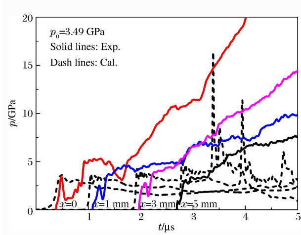
图 6 CL-20/NTO 混合炸药计算与实验结果对比 Fig. 6 Experimental and calculated pressure histories in shock initiation of CL-20/NTO
