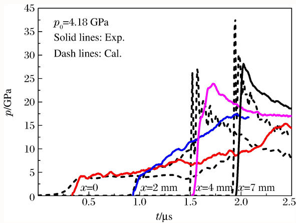
图 5 CL-20 混合炸药计算与实验结果对比 Fig. 5 Experimental and calculated pressure histories in shock initiation of CL-20 explosive
