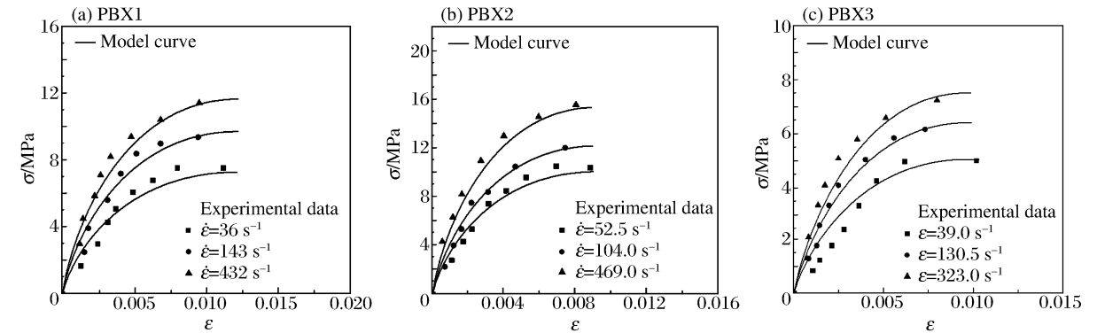
图10 3种炸药动态拉伸本构模型曲线与实验数据的对比 Fig. 10 Comparison between dynamic tension models and experimental data for three explosives
