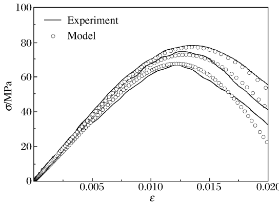
图 5 实验结果与修正的本构模型计算结果的比较 Fig. 5 Comparison between the experimental data and the modified constitutive model
